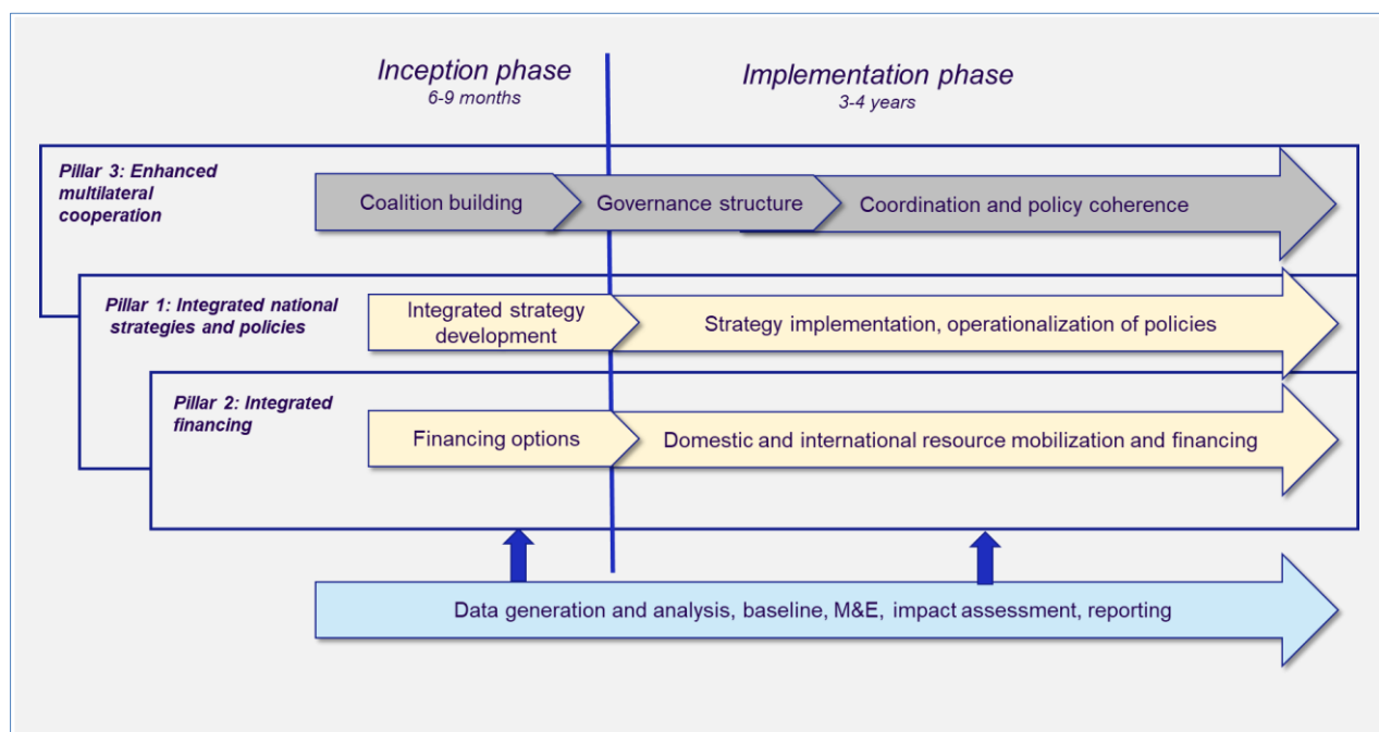
FIGURE 3 Implementation Model
